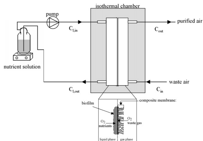
Fig. 1. Membrane bioreactor for removal of waste gas [2]. C_{\text{in}} is the compound's concentration to be treated ( \text{g m}^{-3} ), C_{\text{out}} the purified air ( \text{g m}^{-3} ), and C_{l,\text{in}} and C_{l,\text{out}} are the concentration of nutrients inlet and outlet respectively.
