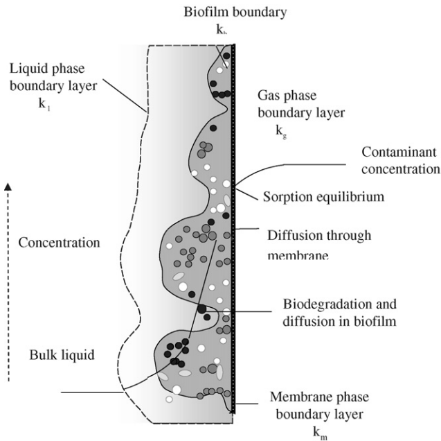
Fig. 2. Mass transfer resistance in a biofilm attached on a flat membrane.
